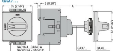
Shaft extensions for door coupling handles GAX7...
