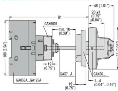
GAX7...A used with GAX60 01 and GAX66/66B
