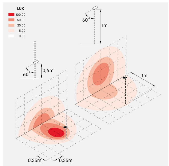
cnc_35_swing_20_optic_D
