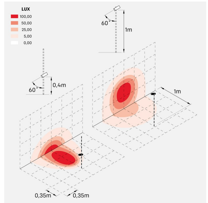
cnc_35_swing_20_honeycomb_optic_M
