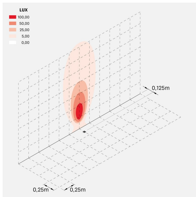
cnc_35q_20_honeycomb_optic_M
