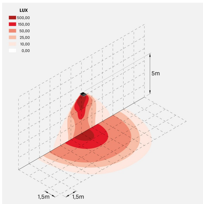
delta3_circular_135W_optic_C1
