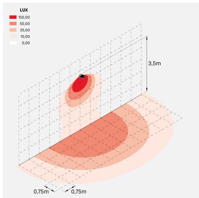
delta0_simm_30W_optic_S1
