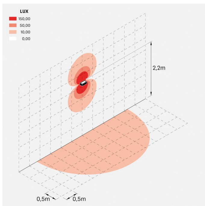
trend_220_15w_ued_poliglass
