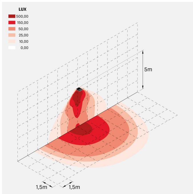
delta3_circular_200W_optic_C1
