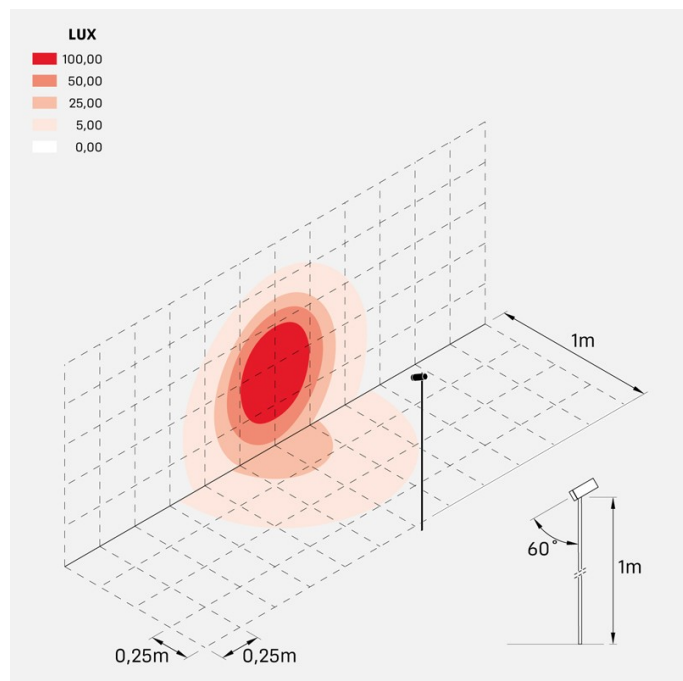
cnc_35_swing_garden100_20_honeycomb_optic_S
