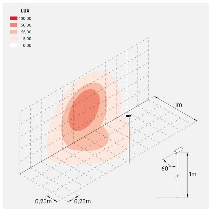
cnc_35_swing_garden100_20_honeycomb_optic_L
