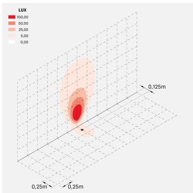
cnc_35t_20_honeycomb_optic_L
