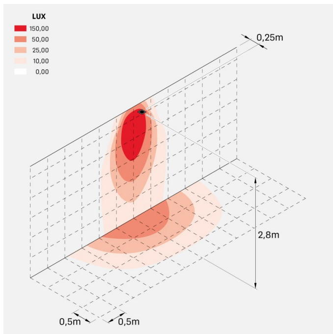
pop_80_asim_q_s
