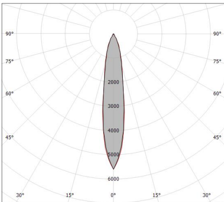
cd/km η = 100% - - C0/C180 - - C90/C270
