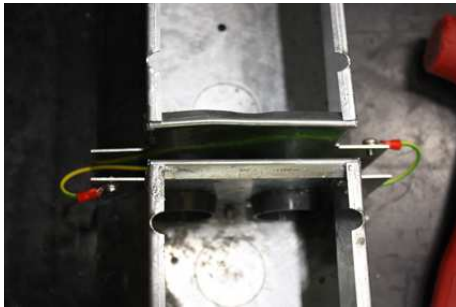
CABLARE LE CONTROCASSE A TERRA WIRE THE OUTERCASING ON THE GROUND
