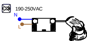
COLLEGAMENTO SINGOLO ON/OFF SINGLE CONNECTION ON/OFF
