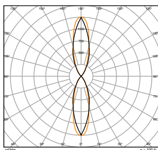
UB WL VARIO SQ 29W ML 840 GY 30D Up Down
