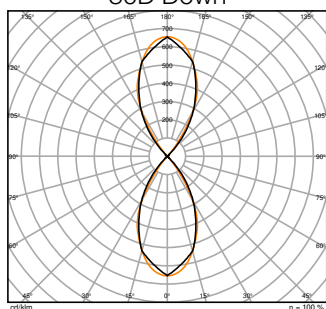
UB WL VARIO SQ 29W ML 840 GY 55D Up Down
