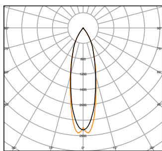
UB WL VARIO SQ 29W ML 827 GY 30D Down
