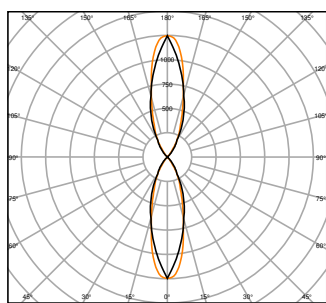
UB WL VARIO SQ 29W ML 827 GY 30D Up Down
