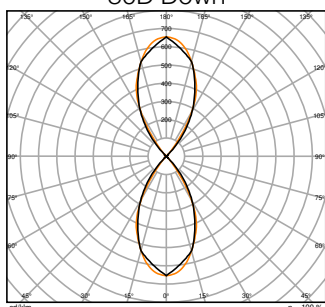
UB WL VARIO RD 29W ML 827 GY 55D Up Down
