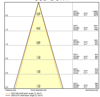
UB WL VARIO RD 29W ML 827 BK 30D Up Down
