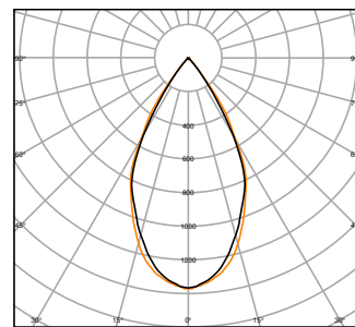
UB WL VARIO RD 29W ML 827 BK 55D Down
