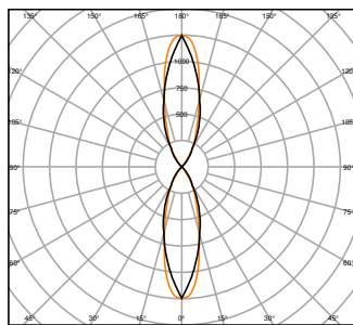
UB WL VARIO RD 29W ML 827 BK 30D Up Down
