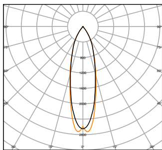
UB WL VARIO RD 29W ML 827 BK 30D Down
