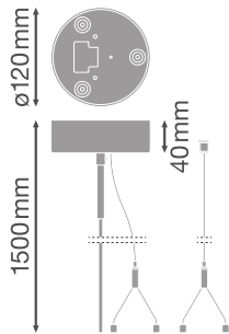
LN INV SUSPENSION KIT
