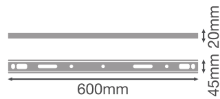
HB FLEX BRACKET CHAIN
