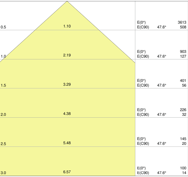
LEDVANCE TruSys LED DALI 53W 4000K WW SI
