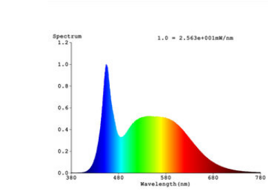
RGBW Remote Lamp 6500K
