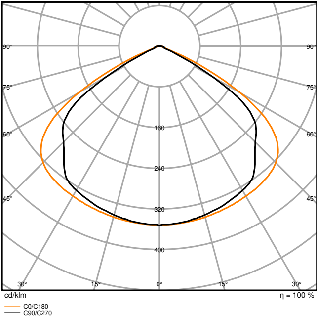
LB FLEX 1500 DALI P 140W 840 VV
