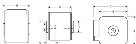
Fusibili serie A-125E con fori filettati (TS) - Series A-125E fuses with threaded holes (TS)
