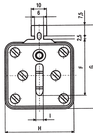
Fusibili NHL grandezza 1-2-3 NHL fuses, sizes 1-2-3
