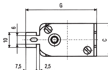
Fusibili NHL grandezza 00-0 NHL fuses, sizes 00-0
