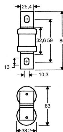
Fusibili tipo W-250GHW Fuse type W-250GHW
