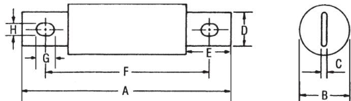
Fusibili 65A÷600A - 65A÷600A fuses
