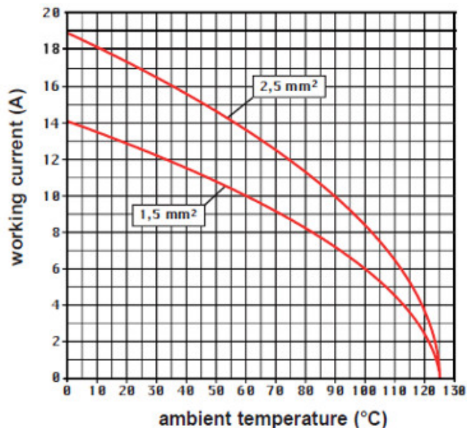
Derating curves
