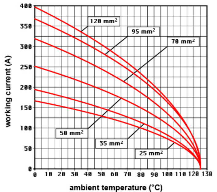
CX 01/01B 30, 1 pole connector inserts Maximum current load derating diagram
