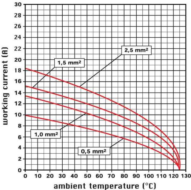
diagram CSH 24 poles
