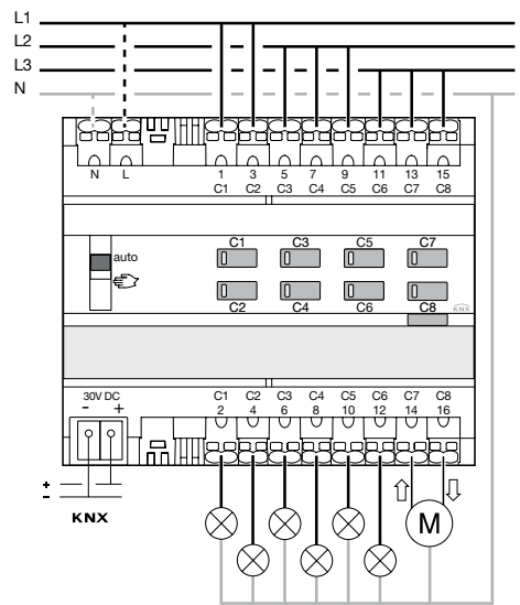
Fig 2: Device connection
