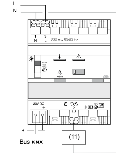
Fig 3: Device connection
