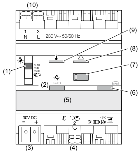
Figure 1: Device overview
