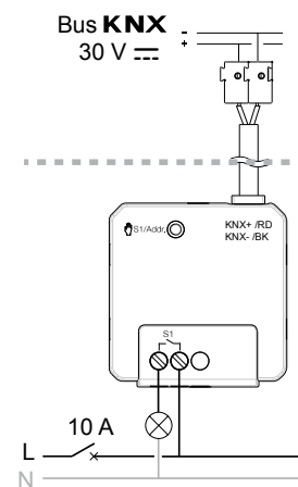
Fig 3: device connection 1gang
