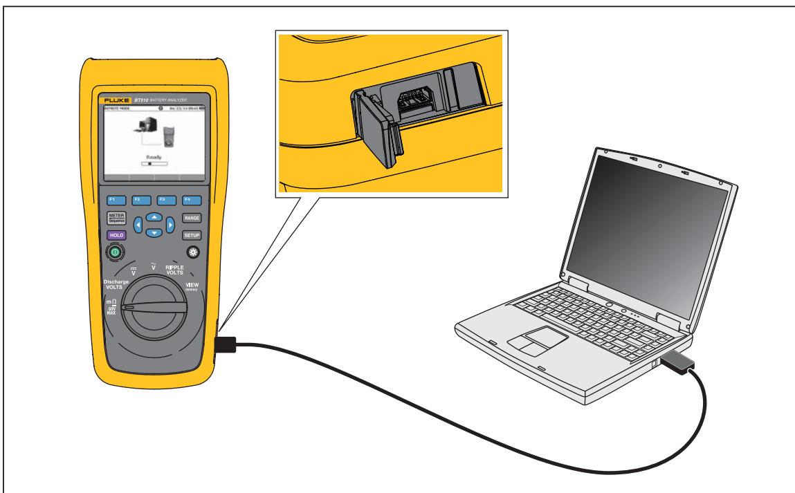
Figure 5-1. Collegamento a PC
