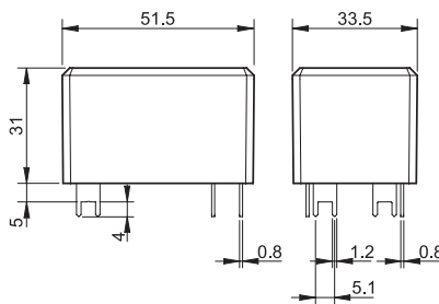
Tipo 66.22-x600S
