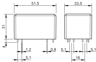
Tipo 66.22-x600S
