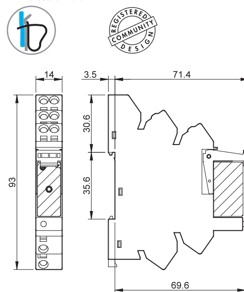
Tipi 38.11 38.41 38.62 Morsetti a molla
