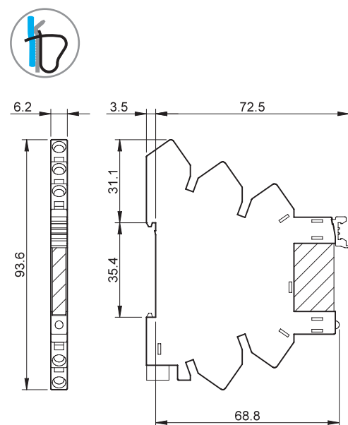
Tipi 38.61 / 38.61.3 38.91 / 38.91.3 Morsetti a molla
