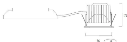
Dimensions (mm)
