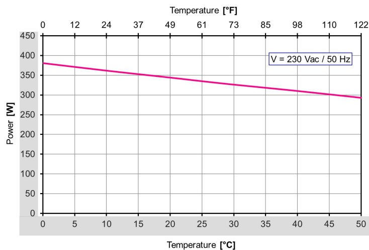
Power-Temperature
