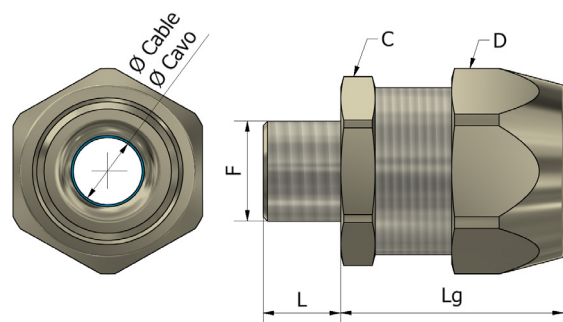
Filetto cilindrico / Cylindrical thread : GAS ISO 228
