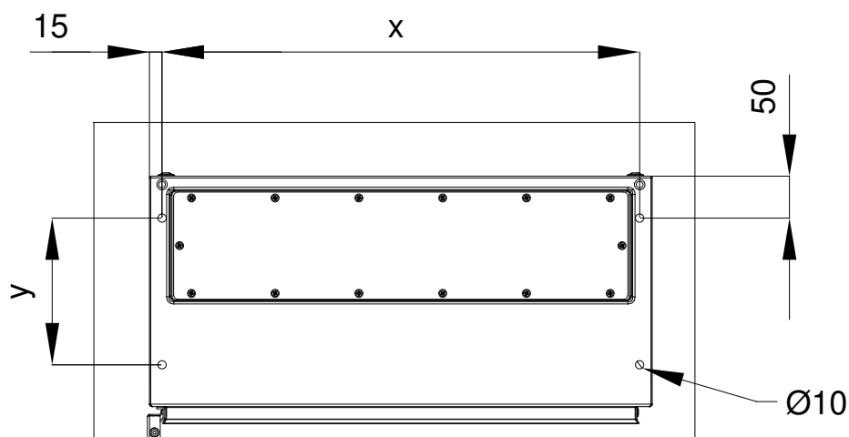
Cut-out dimensions
