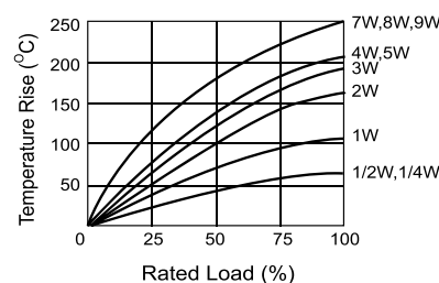
Heat Rise Chart
