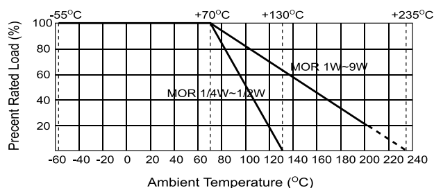
Derating Curve
