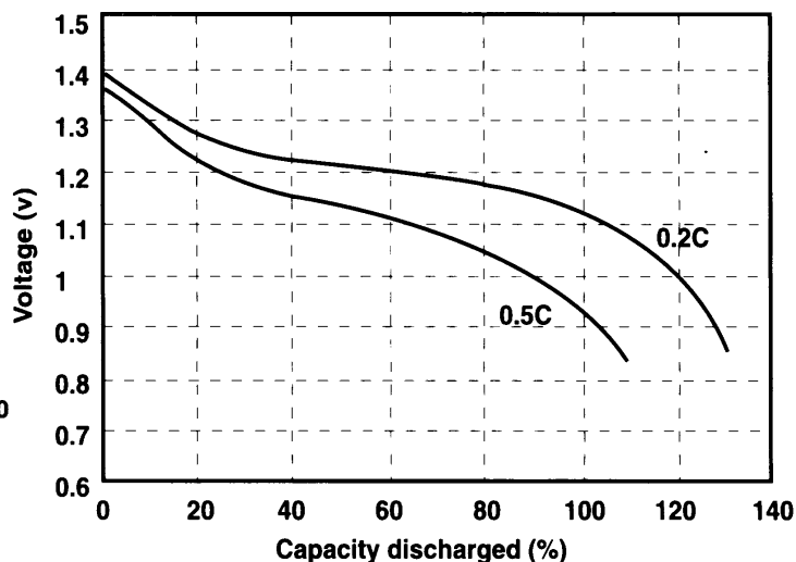
Discharge curves of single cell E-280B26 at various discharge rates at room temperature.
