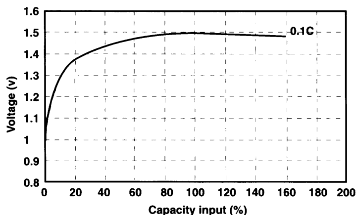
Charging curve of single cell E-280B26 at 0.1C charging rate
