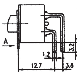
PC-H terminal (3)
