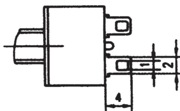
Solder terminal (1)
