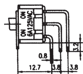
PC-V terminal (4)
