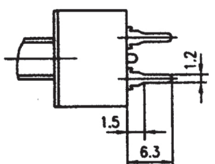
PC terminal (2)
