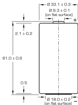
Finished version with protruding positive end cap
