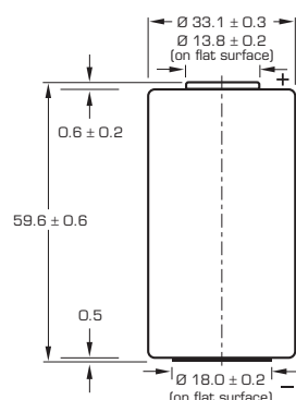
Finished version with flat positive end cap
