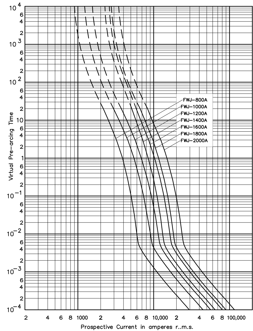
Time-current curve - 800 A to 2000 A
