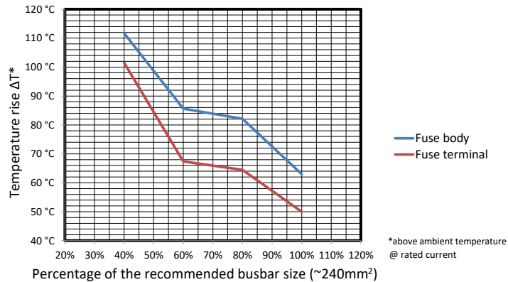
Temperature rise for various busbar sizes
