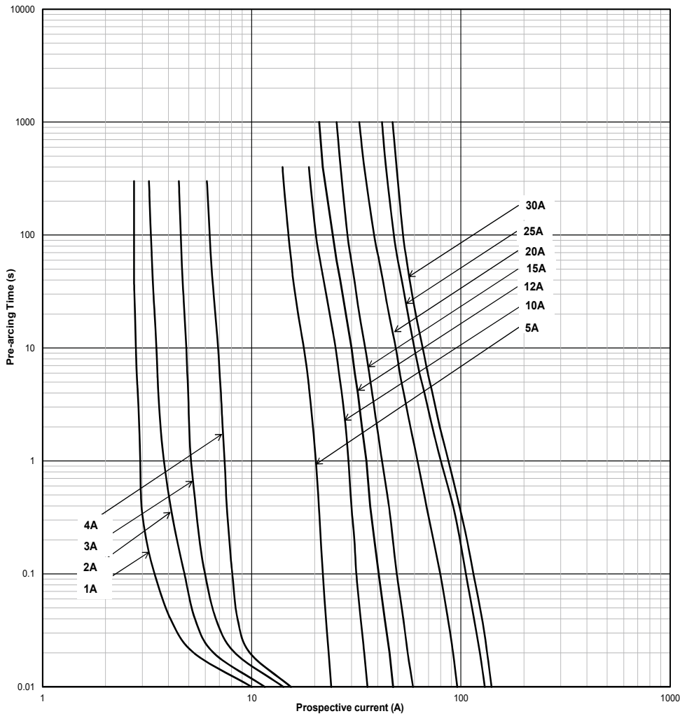
Time-current curve - 1 A to 30 A
