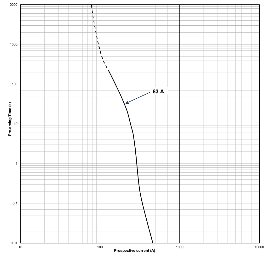
Time-current curve - 63 A
