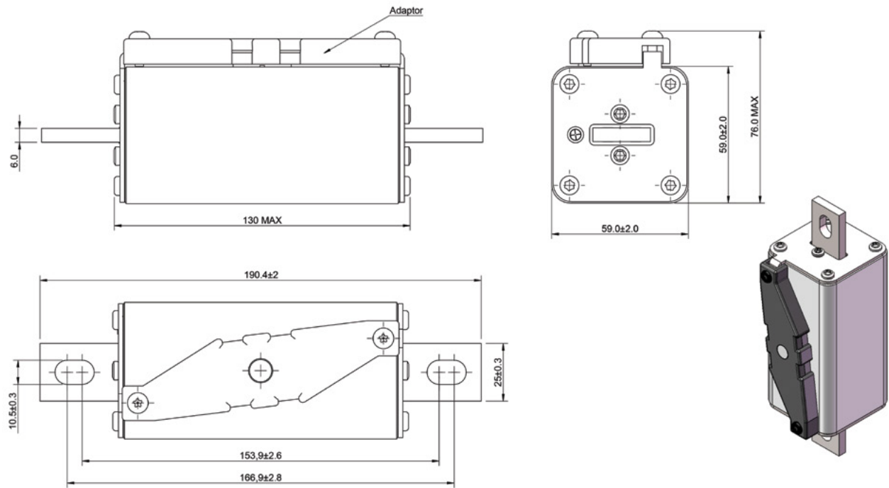
Dimensions (mm) - Size 2, bolted
