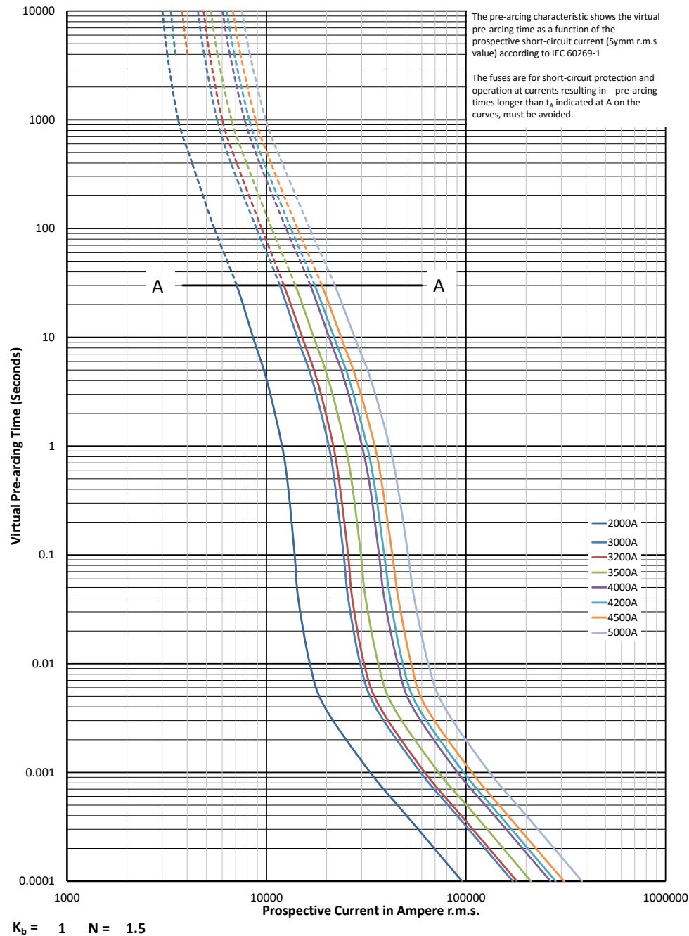
Time-current curve - 2000 A to 5000 A
