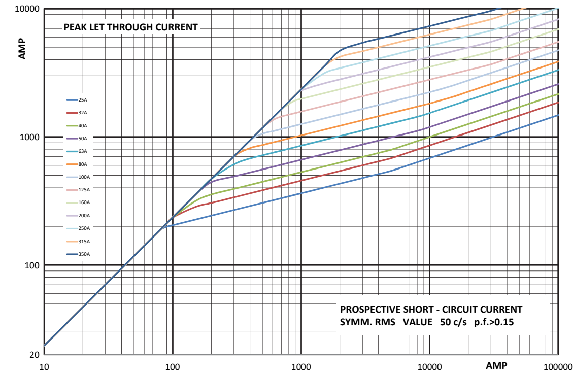
Cut-off curve - Size 000, 25 A to 350 A
