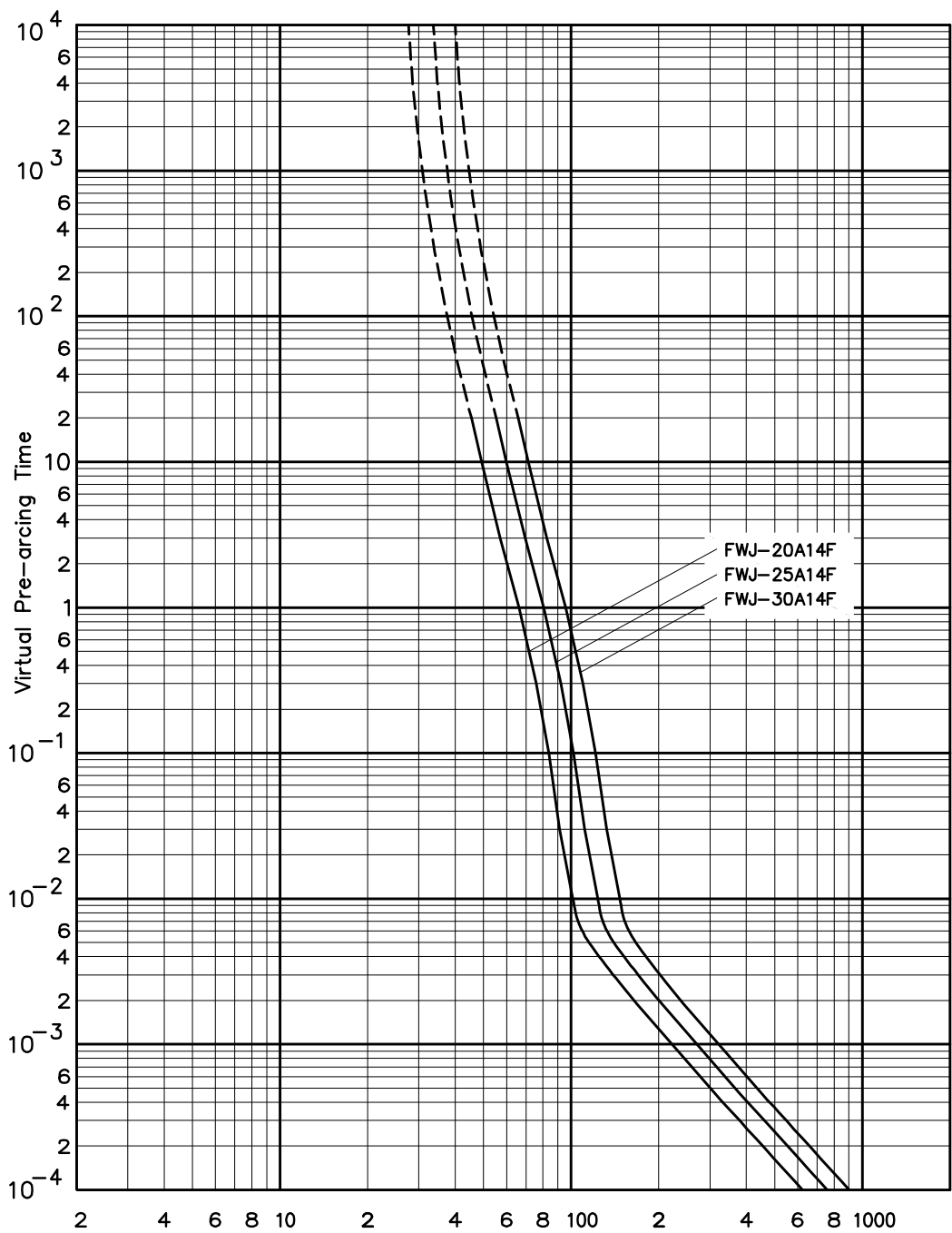
Time-current curve - 20 A to 30 A
