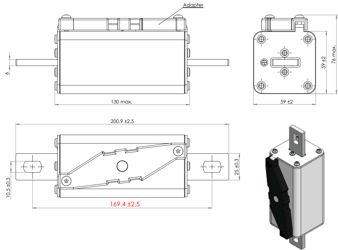
Dimensions (mm) - Size 2XL-3B, bolted
