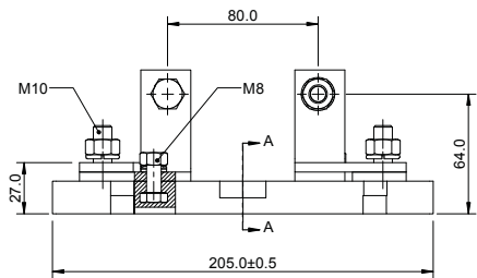
Dimensions (mm) - 170H3004
