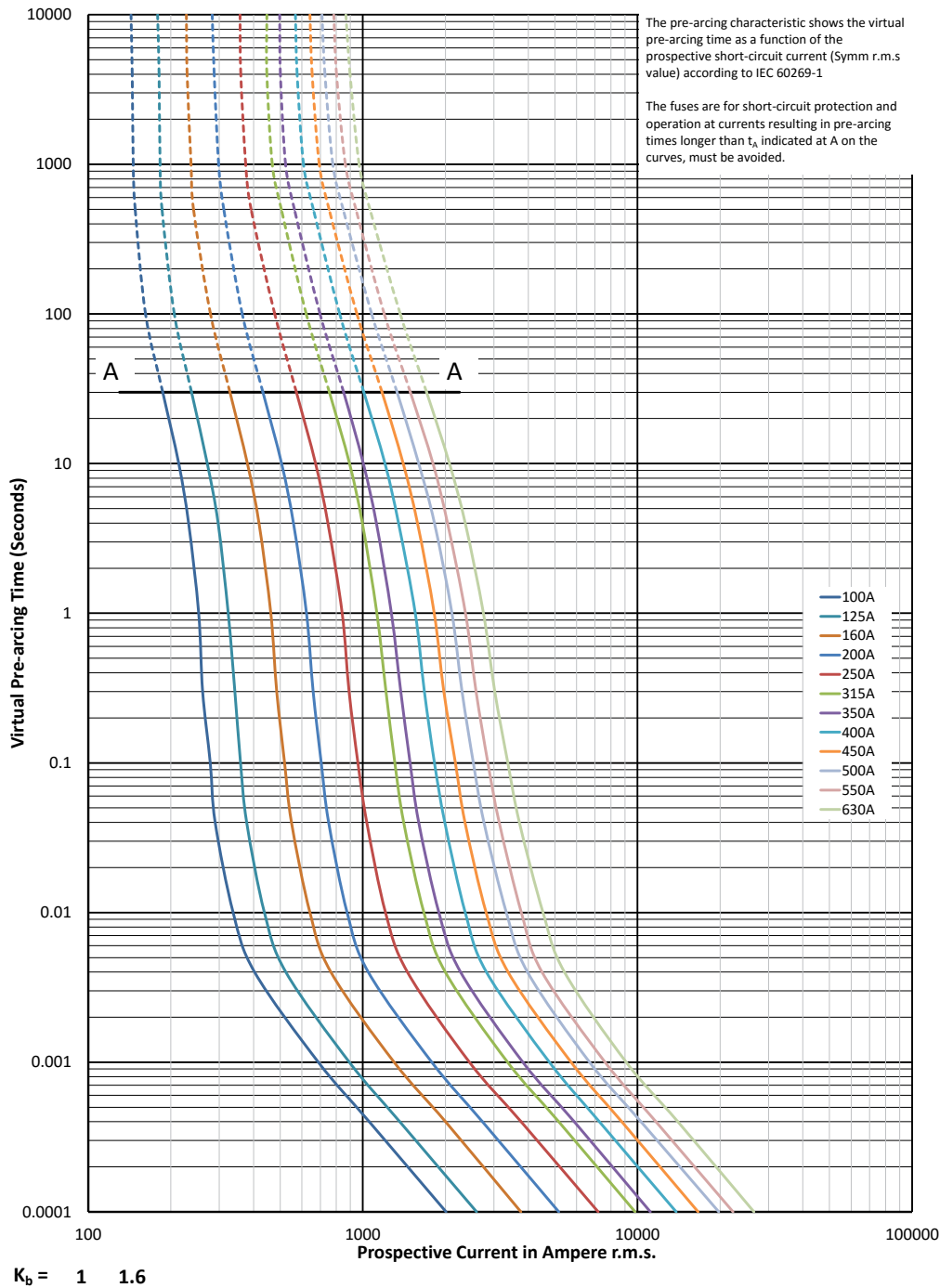
Time-current curve - Size 230, 100 A to 630 A
