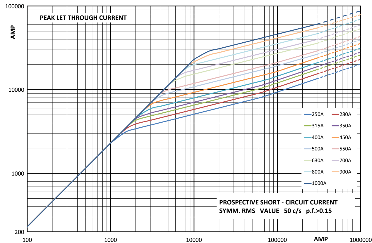
Cut-off curve - Size 2, 250 A to 1000 A
