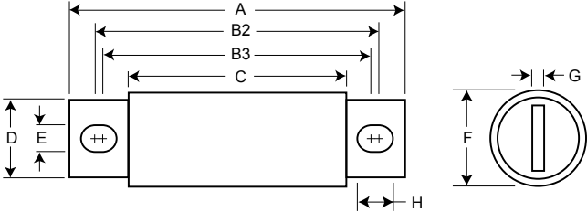
Dimensions (in) - 35 A to 400 A
