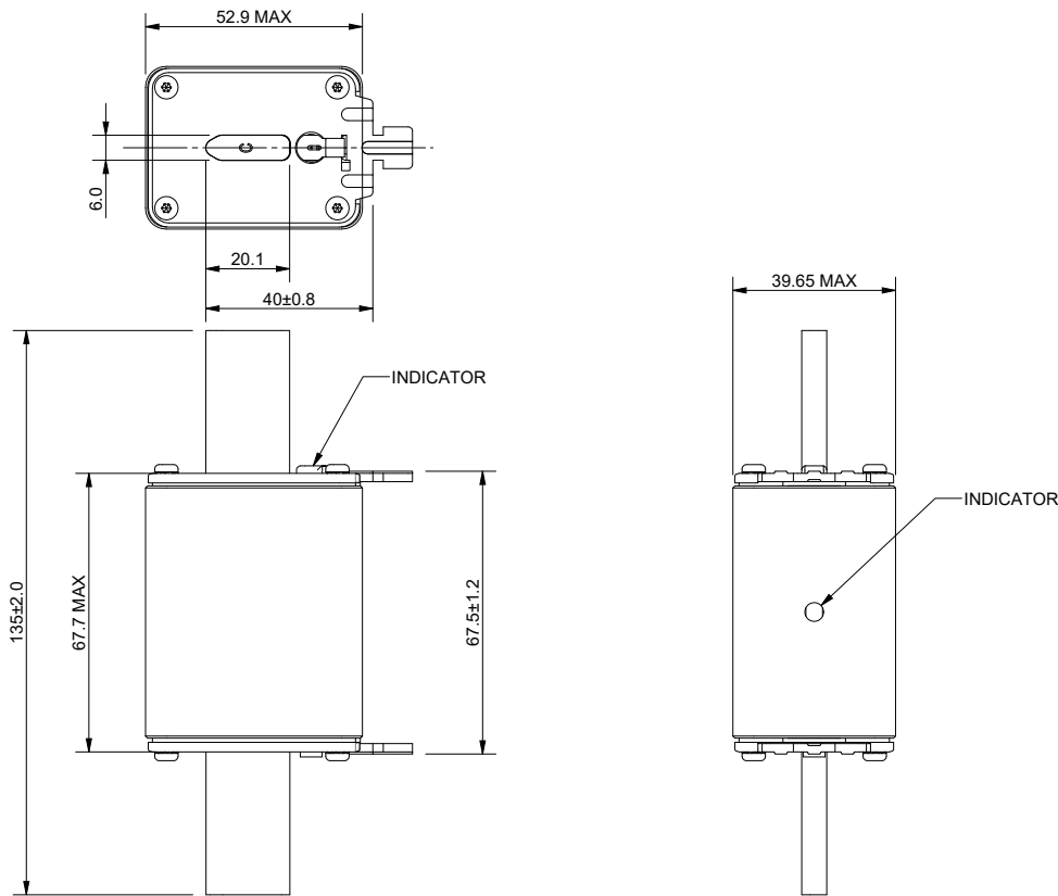
Dimensions (mm) - Size 1, bladed
