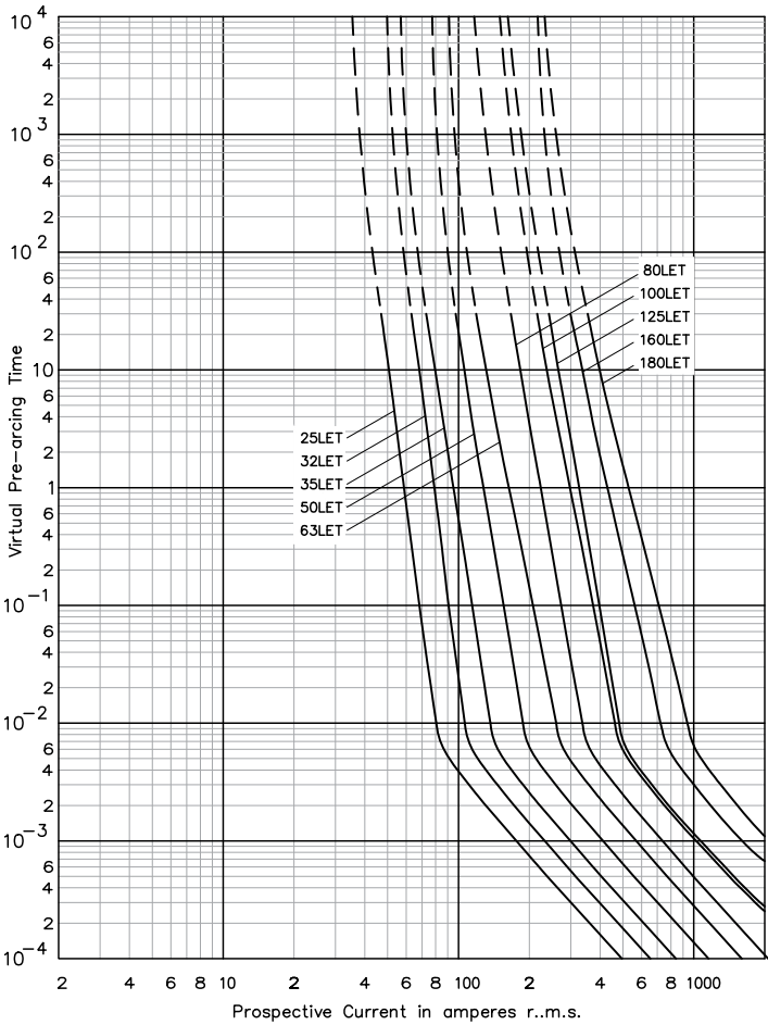
Time-current curve - LET, 25 A to 180 A
