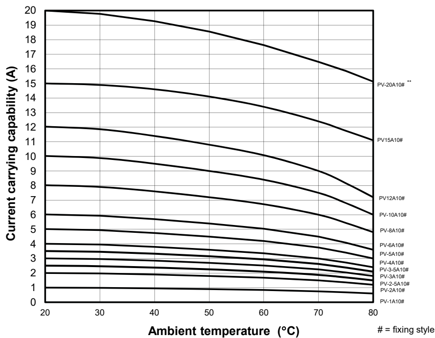
Temperature deratings
