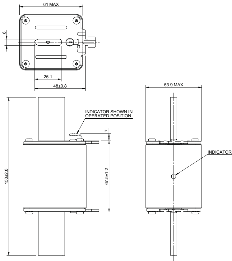
Dimensions (mm) - Size 2, bladed
