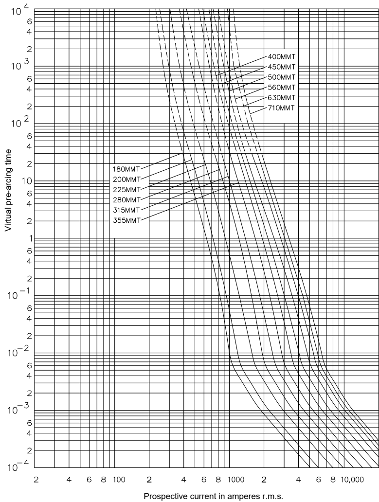
Time-current curve - MMT, 180 A to 710 A
