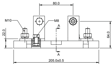
Dimensions (mm) - 170H3003
