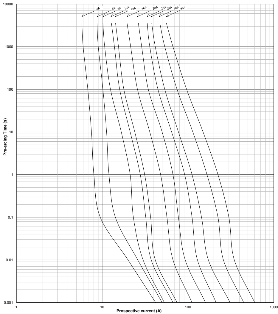
Time-current curve - 4 A to 50 A
