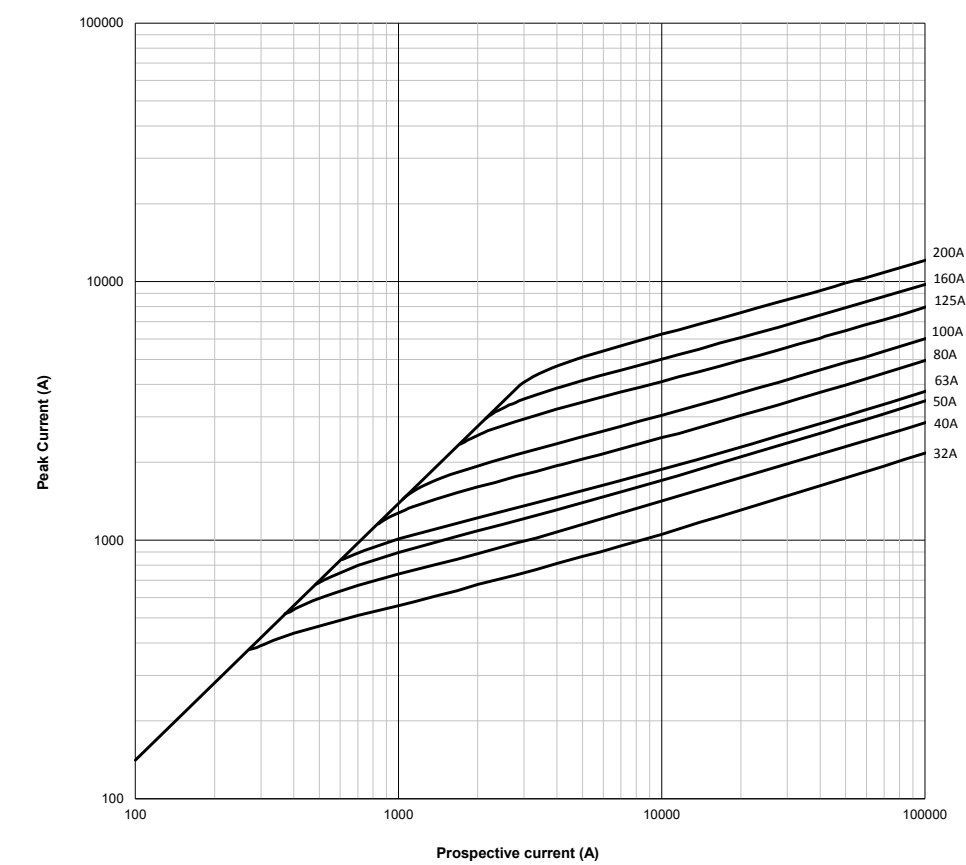
Cut-off curve - Size 1, 32 A to 200 A
