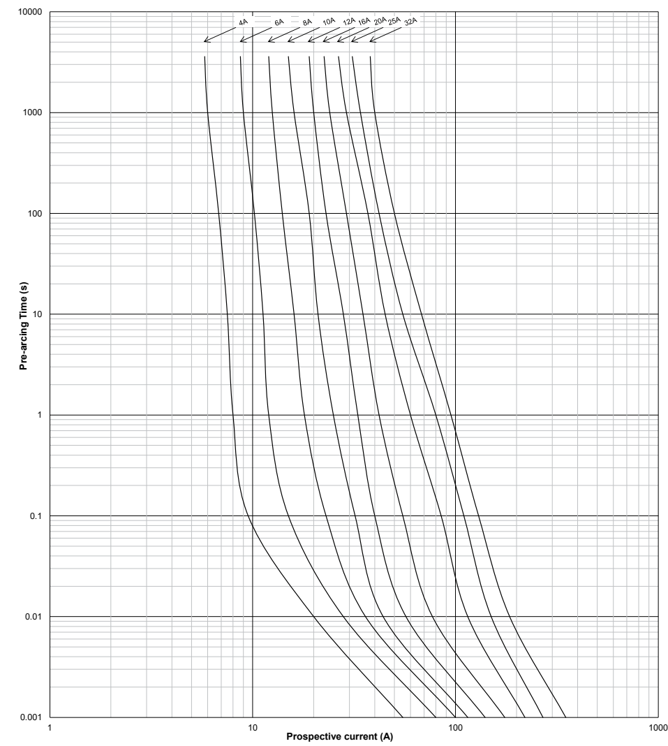
Time-current curve - 4 A to 32 A
