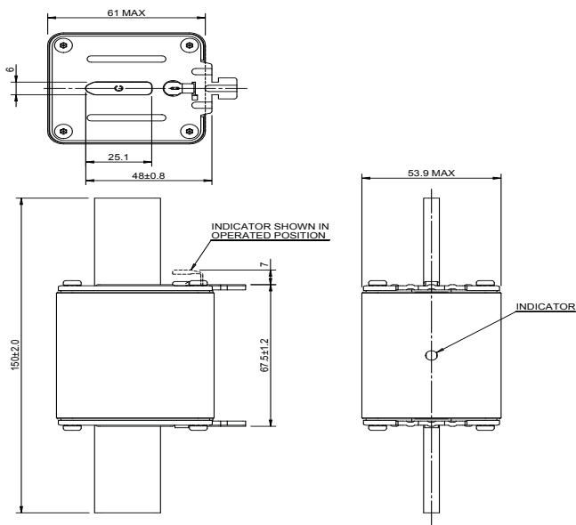
Dimensions (mm) - NH2, bladed with lugs
