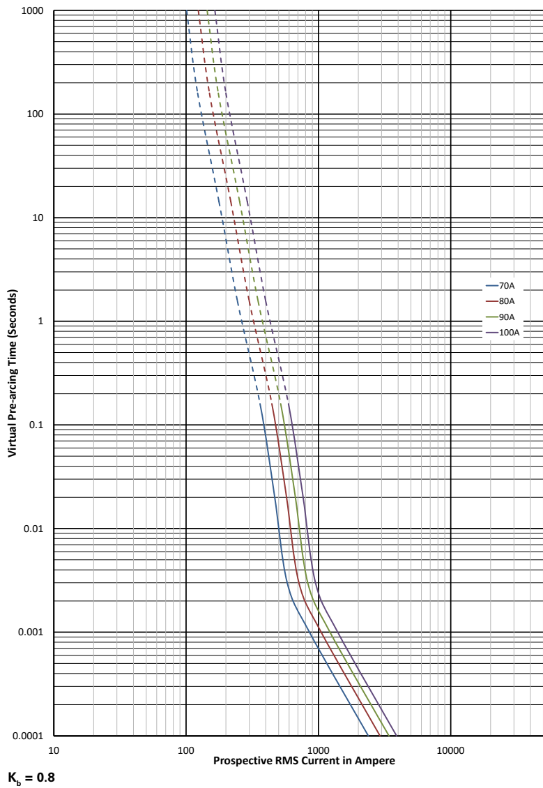
Time-current curve - 70 A to 100 A - 25 mm fuse links
