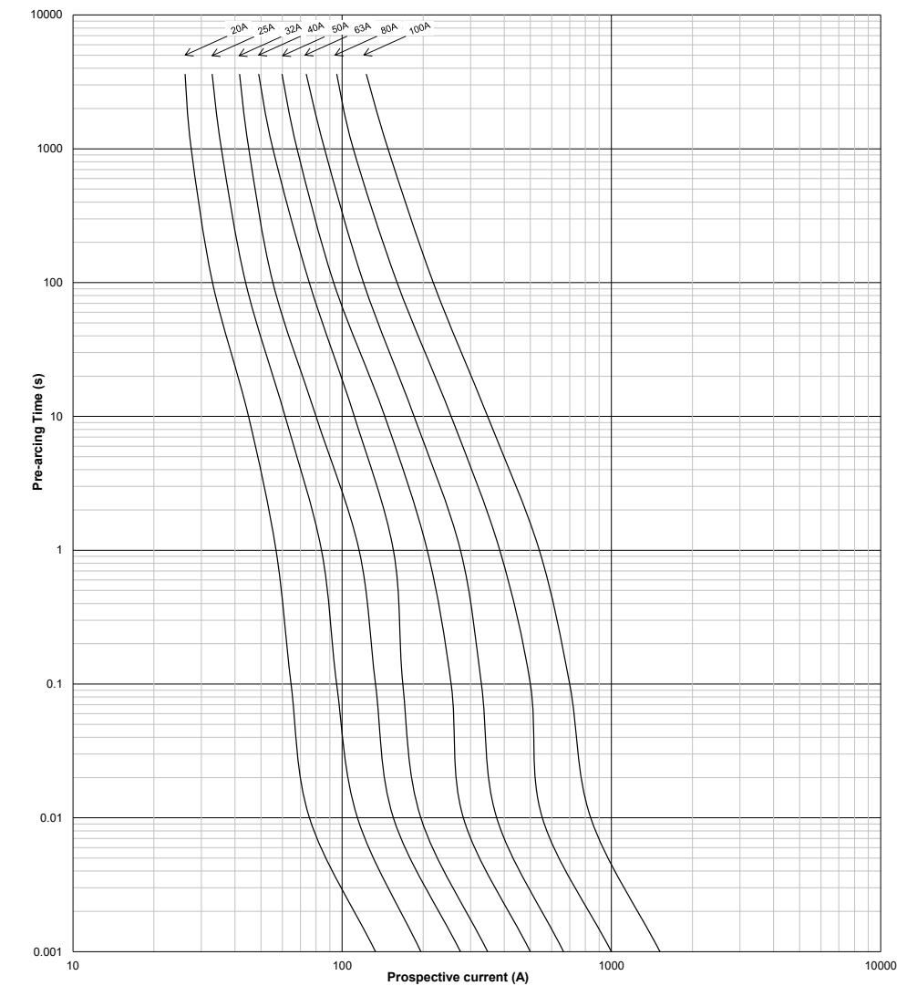
Time-current curve - 20 A to 100 A
