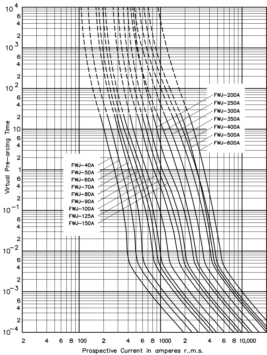
Time-current curve - 35 A to 600 A
