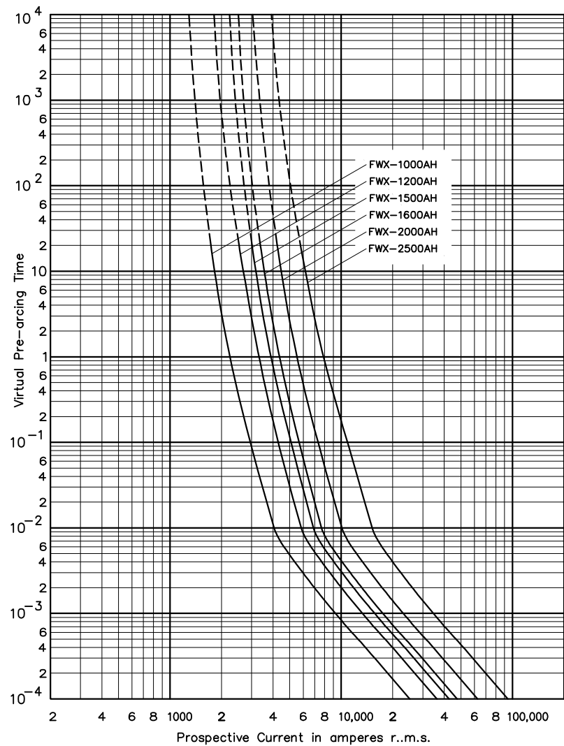
Time-current curve - 1000 A to 2500 A
