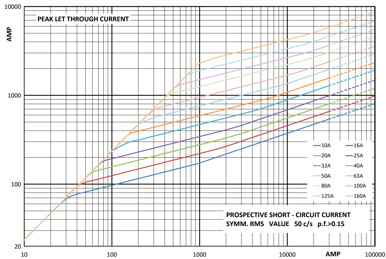
Cut-off curve - Size 00, 10 A to 160 A
