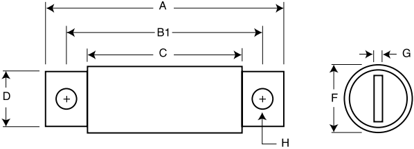
Dimensions (in) - 1 A to 30 A and 450 A to 1000 A
