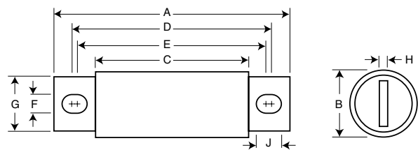
Dimensions (in) - 35 A to 2000 A
