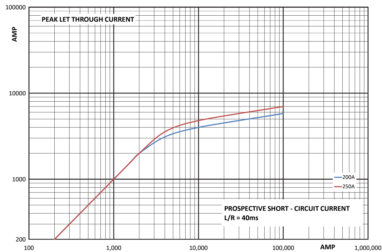
Cut-off curve - Size 1, 200 A and 250 A
