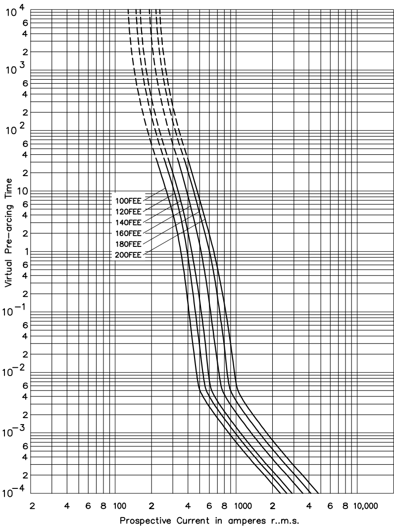
Time-current curve - FEE, 100 A to 200 A
