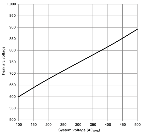
AC Arc Voltage
