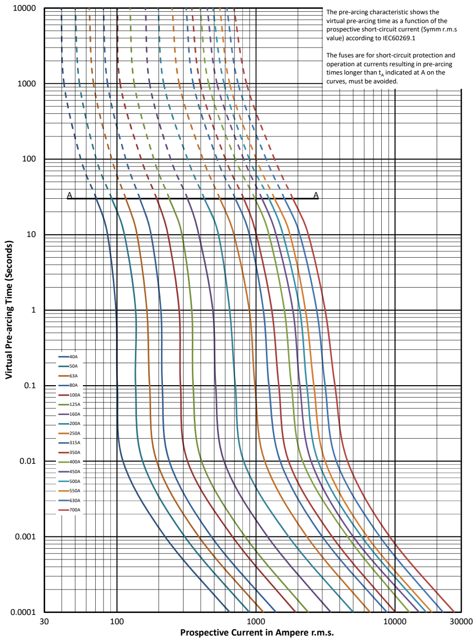
Time-current curve - Size 1, 40 A to 700 A
