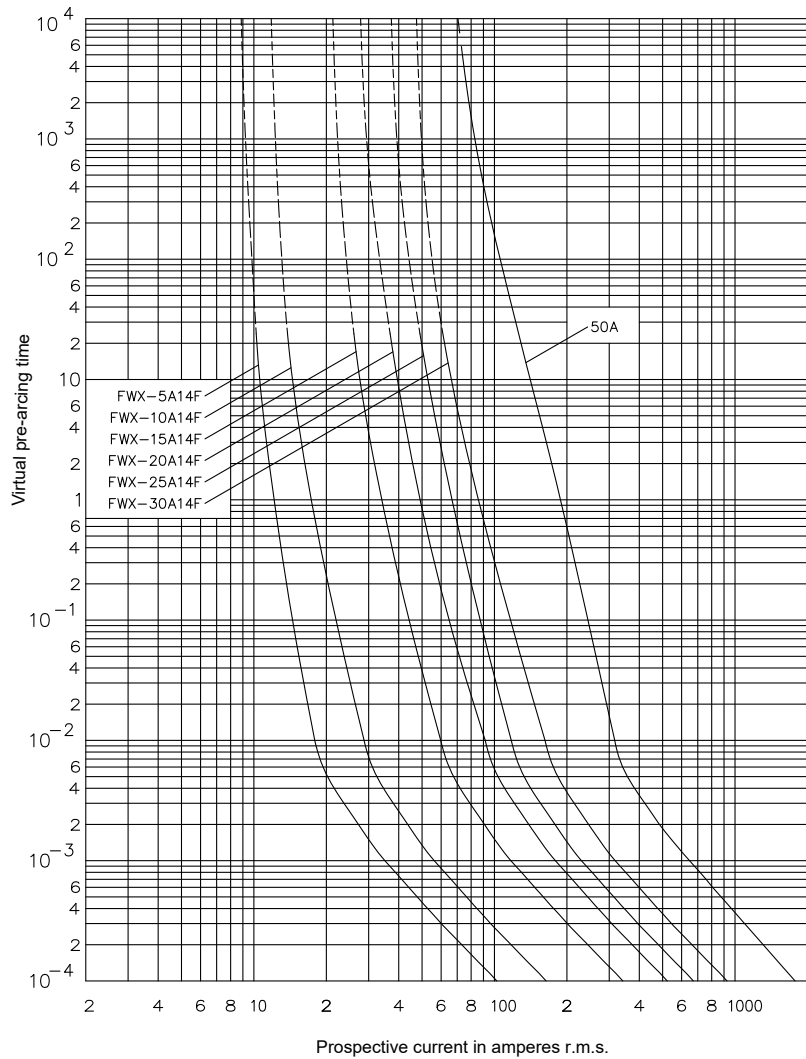
Time-current curve - 5 A to 50 A
