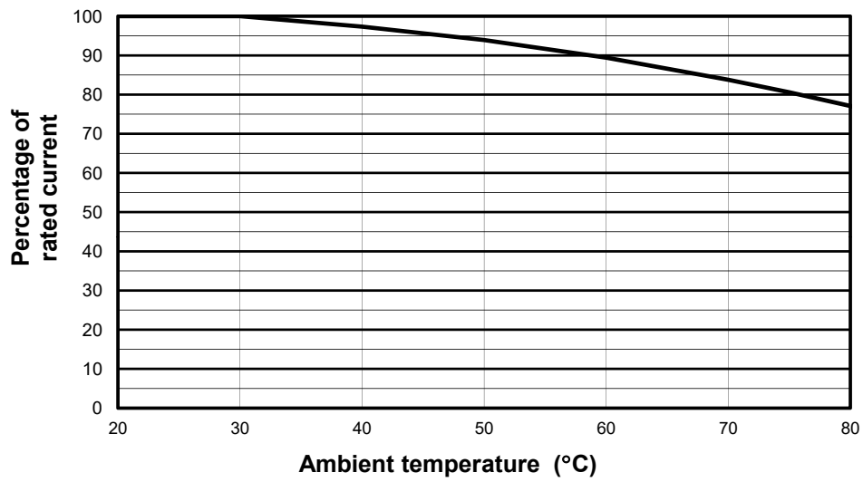
Temperature derating curve
