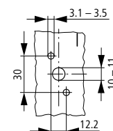
Drilling dimensions
