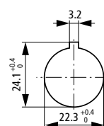
Drilling dimensions
