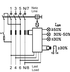
Ä Basic diagram
