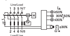
Ä Without use of auxiliary contact line/load side free selectable
