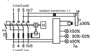
Ä Signalisation with Isolation Transformer 1:1 (IEC/EN 60664)
