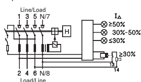
Ä Signalisation without Isolation Transformer 1:1 (IEC/EN 60664)
