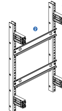
Fig. 3: Fixing of DIN support rails when using the electric shock protection cover plate as a pan 1) Cover plate holder 2) DIN support rail
