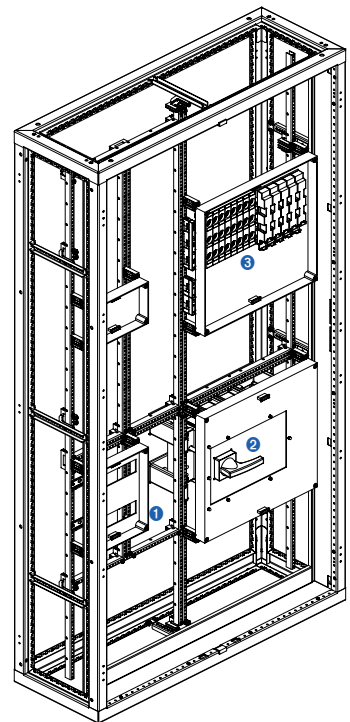
Fig. 1: Cabinet distribution board, partly equipped with standard-section EP fitting-kits 1) Fitting module type EP for DIN-modular components 2) Fitting module type EP for Dumeco load disconnectors 3) Fitting module type EP for busbar-mounting fuses
