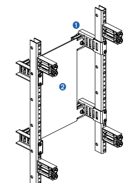
Fig. 8: Mounting plate with a set of drop-down shackles 1) Set of drop-down shackles 2) Mounting plate
