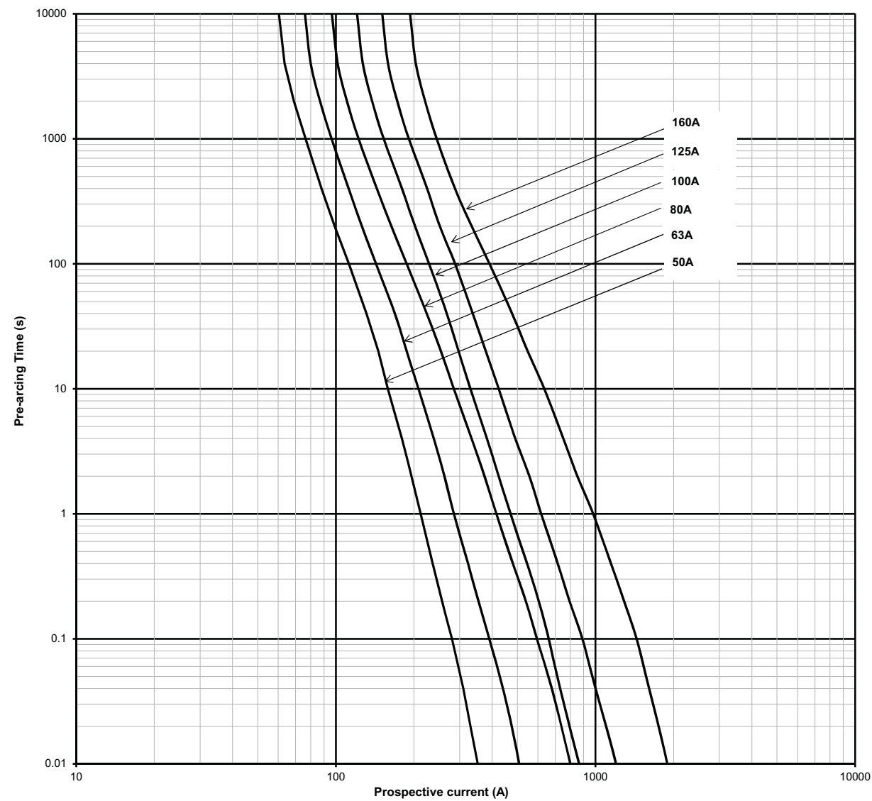
Time current curve - 1500 V d.c. - 01XL - Bladed and bolted
