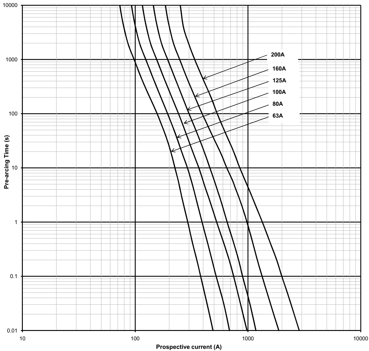
Time current curve - 1000 V d.c. - 01XL - Bladed and bolted
