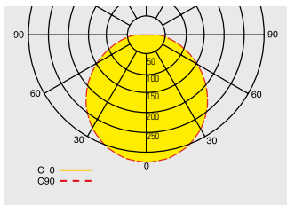
Light distribution curve 83022 LED CG-S
